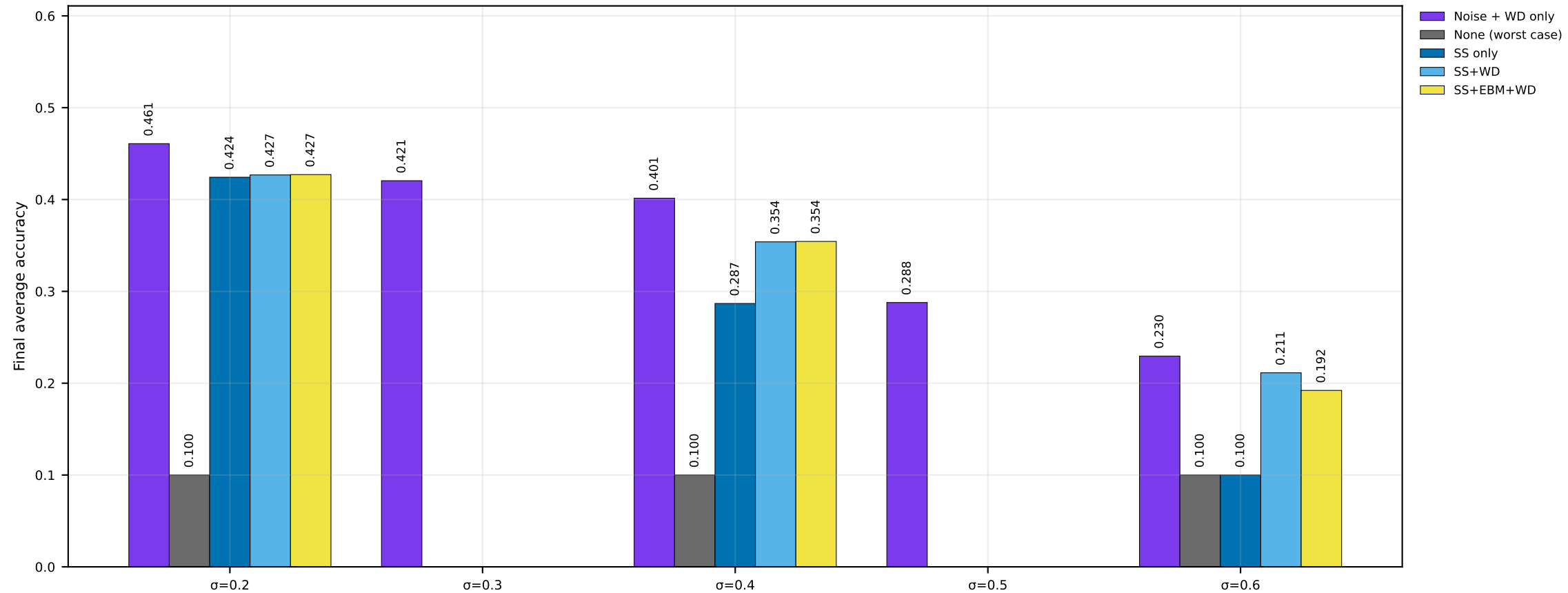
Ablation Groups | CIFAR-10 | MERGED | seed=avg of 4 seeds (nonIID)
